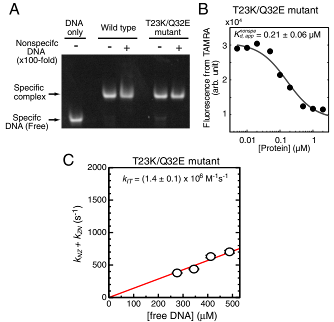
Fig. 6. Impact of T23K/Q32E mutations on DNA-binding specificity, affinity, and intersegment transfer. (A) EMSA competition assay using 100-nM TAMRA-labeled specific 28-bp DNA (the same sequence as 5P28) and 200-nM protein in the absence and presence of 10,000-nM unlabeled 28-bp nonspecific DNA NS28. Protein and DNA were mixed in a buffer of 10 mM Tris•HCl (pH 7.5), 40-mM KCl, and 5% glycerol. Shown results indicate that the T23K/Q32E mutant retains affinity and specificity to the target DNA sequence. (B) Fluorescence-based affinity measurement for the interactions between the T23K/Q32E mutant protein and TAMRA-labeled nonspecific 28-bp DNA (the same sequence as NS28). The experimental conditions are the same as those for Fig. 1B. (D) Kinetics of intermolecular translocation of the T23K/Q32E mutant between nonspecific DNA duplexes. The experimental conditions are the same those for Fig. 4B. For the sake of comparison, the kinetic data are shown on the same scale as that for Fig. 4B. Intersegment transfer of the T23K/Q32E mutant protein is 2.6-fold slower than that of the wild type protein.
