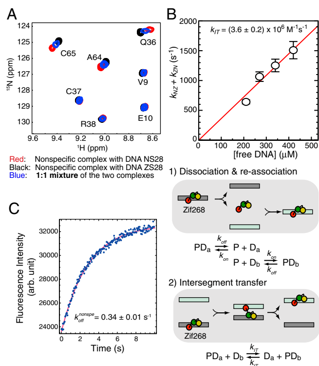
Fig. 4. Translocation kinetics for Egr-1 bound to nonspecific DNA. (A) Overlay of TROSY spectra recorded for two nonspecific complexes of Egr-1 (with DNA NS28 or ZS28) and a 1:1 mixture of the two complexes. ZS28 is a 28-bp DNA duplex with a sequence of 5'-GTACCGATAGACGTTTCCGAACCTTCAG-3'. Egr-1's translocation between the two nonspecific DNA duplexes occurs in a fast exchange regime. (B) Sum of pseudo first-order rate constants for Egr-1's translocation between two nonspecific DNA duplexes NS28 and ZS28 ( k_{NZ} + k_{ZN} ). The rate constants were calculated by global fitting to NMR line-shape data for amide resonances of Q36, F44, I54, E60, C65, K71, and I84, as described previously (16). These residues exhibit a relatively large chemical shift difference ( >35 Hz) for the two nonspecific complexes. (C) Stopped-flow kinetics data for determination of the dissociation rate constant k_{off} for the nonspecific complex of Egr-1 with NS28. Fluorescence arising from TAMRA conjugated to DNA was monitored immediately after the nonspecific complex with TAMRA-labeled DNA NS28 (40 nM) was mixed with unlabeled DNA NS28 (2,000 nM). The rate constant for intersegment transfer ( k_{IT} ) was determined from the DNA-concentration dependence of the apparent rate constants for translocation, together with the k_{off} constant.
