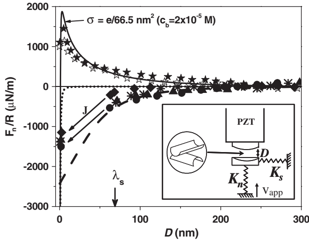
FIG. 1. Normal force profiles F_n(D)/R between curved mica surfaces (mean radius R ) across water with no added salt. \star, \star : interactions between bare mica surfaces (from independent experiments, i.e., different pairs of mica sheets). The solid curve is the prediction based on the PB equation [Eq. (1)] with constant surface charge density \sigma_- = e/(66.5 \text{ nm}^2) , a 1:1 electrolyte concentration c_b = 2 \times 10^{-5} M (derived from the Debye screening length at D \gg \lambda_s ) and a vdW attraction F_{\text{vdW}}(D)/R = -A/6D^2 , with A = 2 \times 10^{-20} \text{ J} . Solid black symbols (from different experiments and contact points): interactions between a chitosan-coated and a bare mica surface; the arrows indicate the jump-in (J) at the point of mechanical instability, expected for (\partial F_n / \partial D) \geq K_n . Broken curve: predicted interaction [4,12] based on antisymmetric surface charge densities, \sigma_+ = |\sigma_-| = e/(66.5 \text{ nm}^2) . Dotted curve: vdW attraction F_{\text{vdW}}(D)/R = -A/6D^2 , with A = 2 \times 10^{-20} \text{ J} . (asterisks and diamonds: 2nd approach of surfaces at 2 different contact points in different experiments; circles and triangles: 1st and 6th approaches, respectively, at a given contact point in a different experiment). The inset shows the schematic of the SFB with the two surfaces facing each other in a crossed-cylinder configuration; K_n and K_s are the constants of the normal and shear springs, respectively, PZT is the sectorized piezocrystal, and v_{\text{app}} the applied velocity of the normal spring mount (bottom) in the dynamic mode [see Eq. (2)].
