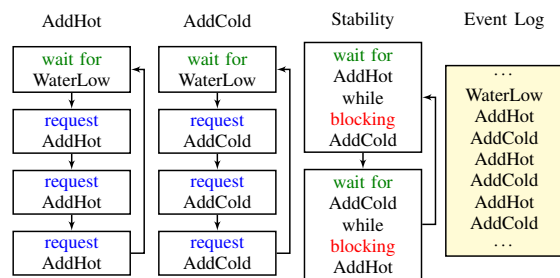
Figure 1: (From (Harel et al., 2014)) Incremental development of a system for controlling water level in a tank with hot and cold water sources. The b-thread AddHot repeatedly waits for WaterLow events and requests three times the event AddHot. AddCold performs a similar action with the event AddCold, capturing a separate requirement, which was introduced when adding three water quantities for every sensor reading proved to be insufficient. When AddHot and AddCold run simultaneously, with the first at a higher priority, the runs will include three consecutive AddHot events followed by three AddCold events. When a new requirement is introduced, to the effect that that water temperature be kept stable, the b-thread Stability is added, enforcing the interleaving of AddHot and AddCold events by using event blocking.
