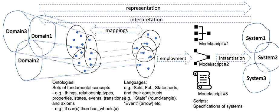
Fig. 1. From real-world problem domains to systems: Left to right (representation): application domains, formalization of concepts within these domains, representation of the formalization as entities in specification languages, programs/scripts/specifications that encode systems structure and behavior, systems. The inverse direction reflects the interpretation of systems and their specifications as real-world effects. Such artifacts can be scanned for indications of hidden assumptions at various levels of abstraction.
