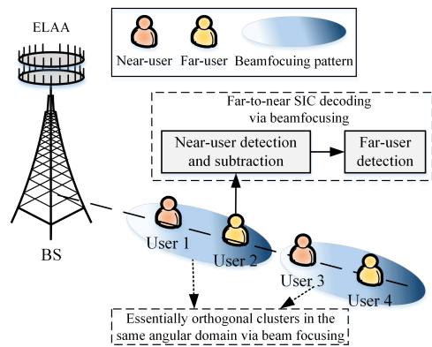
Fig. 7: Illustration of near-field beamfocusing-empowered NOMA, where the near-field beamfocusing vectors divide users in the same angular direction into two clusters and the signal energy is focused on the far-user in each cluster.
