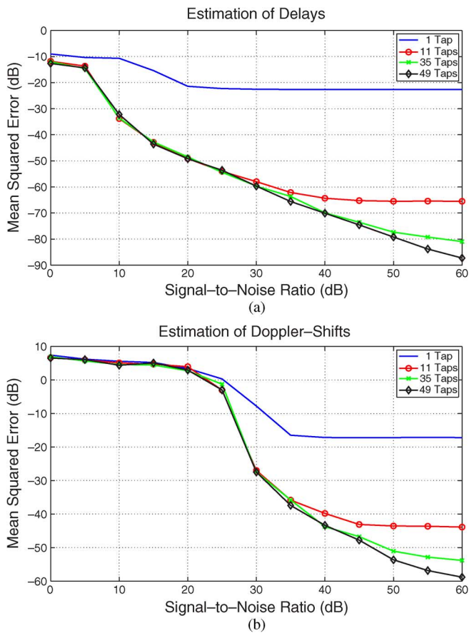
Fig. 7. Mean-squared error of the estimated delays and Doppler-shifts as a function of the signal-to-noise ratio for various lengths of the impulse responses of the filters.
