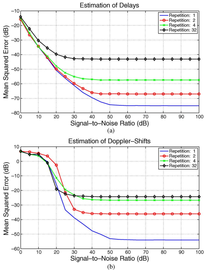
Fig. 11. Mean-squared error of the estimated delays and Doppler-shifts as a function of the signal-to-noise ratio for various probing sequences.
