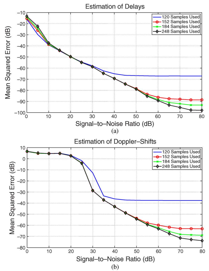
Fig. 8. Mean-squared error of the estimated delays and Doppler-shifts as a function of the signal-to-noise ratio for different numbers of samples collected at the output of the sampling filter (corresponding to an ideal low-pass filter).
