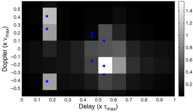
Fig. 3. Quantized representation of nine targets (represented by * ) in the delay-Doppler space with \tau_{\max} = 10 \mu\text{s} and \nu_{\max} = 10 \text{kHz} . The quantized delay-Doppler approximation of the targets corresponds to \mathcal{W} = 1.2 \text{MHz} and T = 0.48 \text{ms} .
