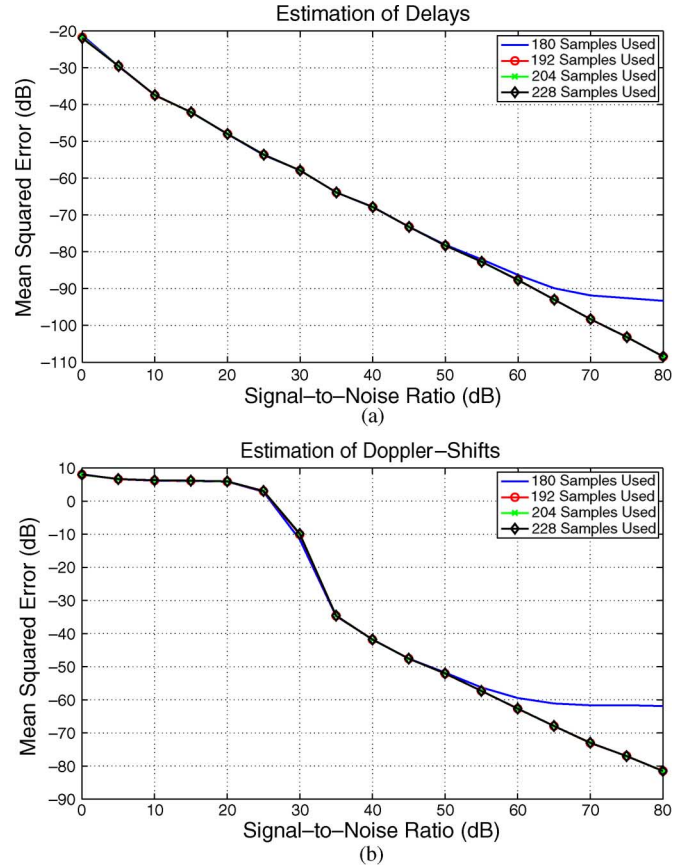
Fig. 10. Mean-squared error of the estimated delays and Doppler-shifts as a function of the signal-to-noise ratio for different numbers of samples collected at the output of a raised-cosine sampling filter with roll-off factor 1.
