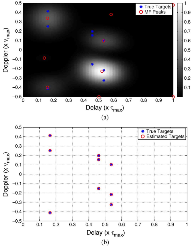
Fig. 4. Comparison between the target-detection performance of matched-filtering and our proposed recovery procedure for the case of nine targets (represented by * ) in the delay-Doppler space with \tau_{\max} = 10 \mu\text{s} , \nu_{\max} = 10 \text{ kHz} , \mathcal{W} = 1.2 \text{ MHz} , and T = 0.48 \text{ ms} . The sequence \{x_n\} corresponds to a random binary ( \pm 1 ) sequence with N = 48 , the pulse g(t) is designed to have a nearly-flat frequency response in the working spectral band \mathcal{F} , and the pulse repetition interval is taken to be T = 10 \mu\text{s} . (a) Target detection by matched-filtering the received signal \mathcal{H}(x(t)) with the input signal x(t) . (b) Target detection using the proposed recovery procedure with p = 12 .
